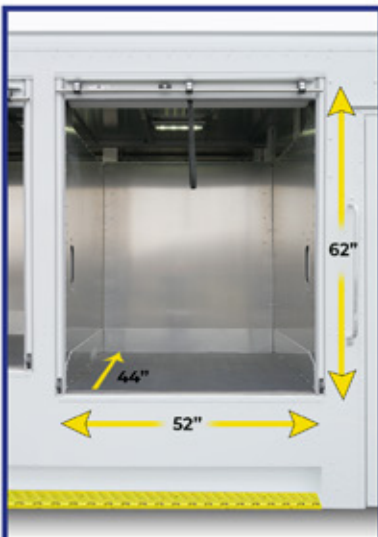
Bay Dimensions
